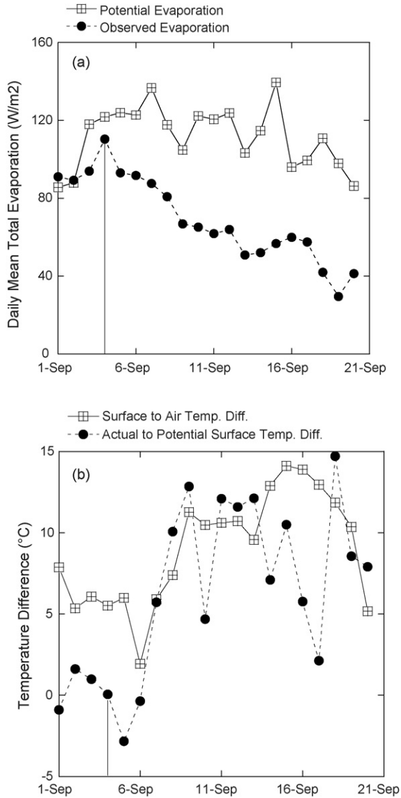
Fig. 3. Same as Fig. 1 in the case of the SALSIA grassland site at maximum development.
